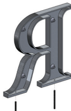
3C - Bottom or Top Stud Letters 4"-24", Minimum 3/8" thick Letters over 8" may require tie-back (not supplied).
